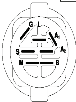
IGNITION SWITCH
