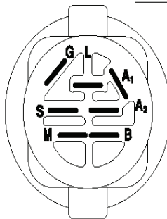
IGNITION SWITCH
