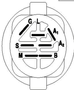
IGNITION SWITCH
